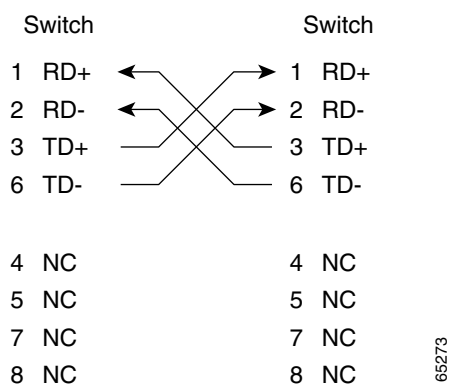
Figure 1-2 Twisted-Pair 10/100BASE-T Cable Schematic
