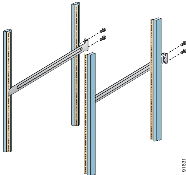
Figure 2-1 Installing the Slider Rails
