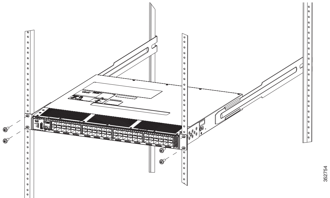
Figure 2-3 Attaching the Switch to the Rack
